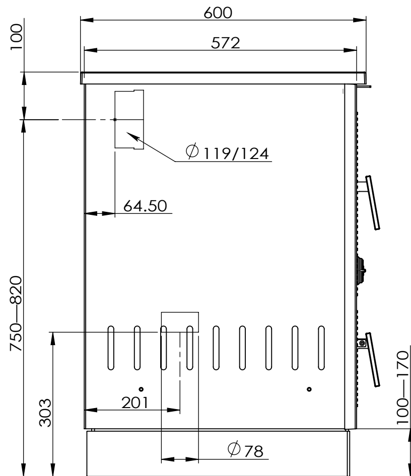
Connection for outdoor air. Connection sleeve for outdoor air. \phi 78
