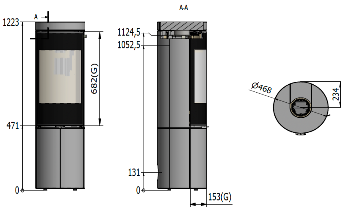
JUNO L 120 (SST + PS) without side glass Dimensions drawing
